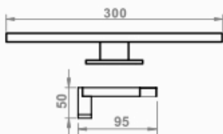
ANNA LED 30 IP 44
