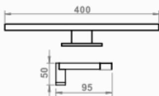
ANNA LED 40 IP 44
